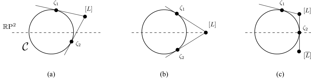
FIGURE 1. Distinct types of [L] \in P(\mathfrak{g}_{\mathbb{C}}) for G = \mathrm{SL}_2(\mathbb{R}) : (a) regular ; (b) real ; (c) non-real degenerate. See the proofs of Lemma 4.1, 4.2 and Remark 4.1.
